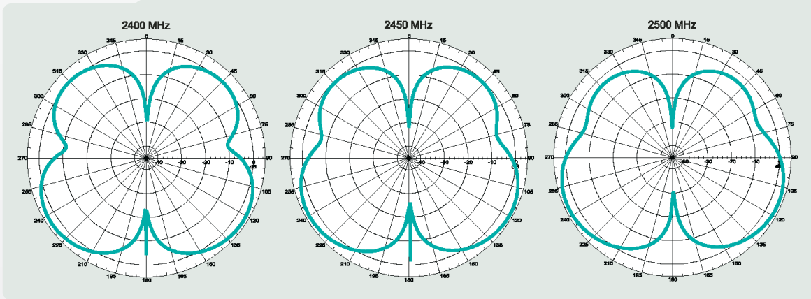
Figure 4: Pulse W107 Antenna Gain Performance
